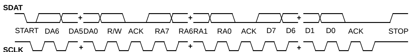
Figure 16. Frame Format (Device Address, R/\bar{W} , Register Address, Register Data)
