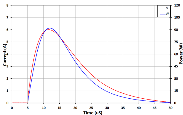
Figure 6-7. Negative Surge Waveform 8 to 20 \mu s
