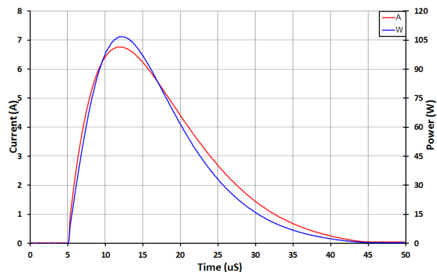
Figure 6-6. Positive Surge Waveform 8 to 20 \mu s
