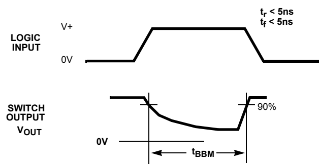
FIGURE 2A. t_{BBM} MEASUREMENT POINTS
