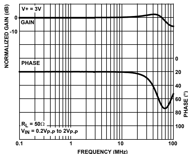
FIGURE 12. FREQUENCY RESPONSE
