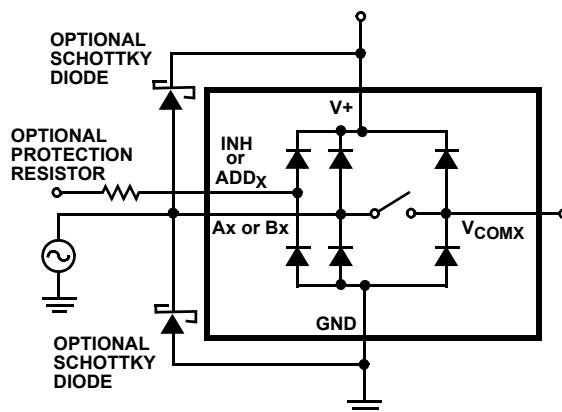
FIGURE 7. OVERVOLTAGE PROTECTION
