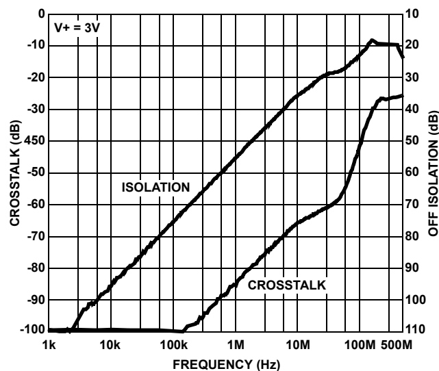
FIGURE 11. CROSSTALK AND OFF ISOLATION
