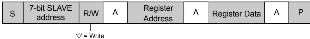
I 2 C Register Read Cycle
