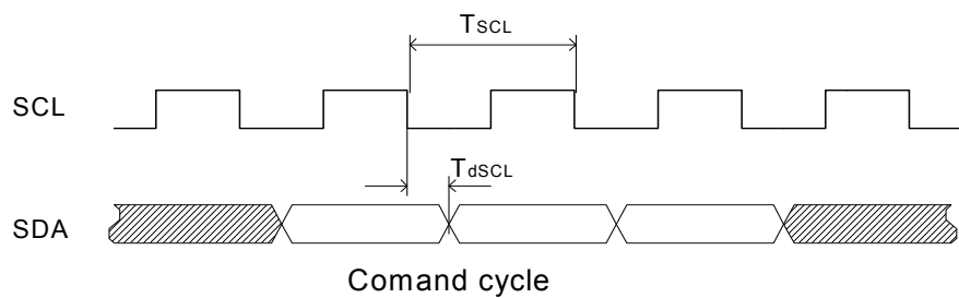
Figure 10 EEPROM Command Cycle Timing Diagram
