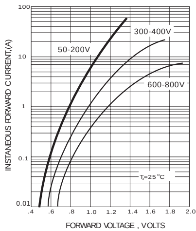
Fig.2- FORWARD CHARACTERISTICS
