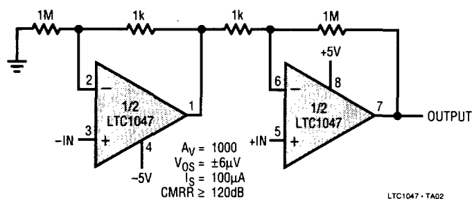
Low Offset, Low Drift Instrumentation Amplifier
