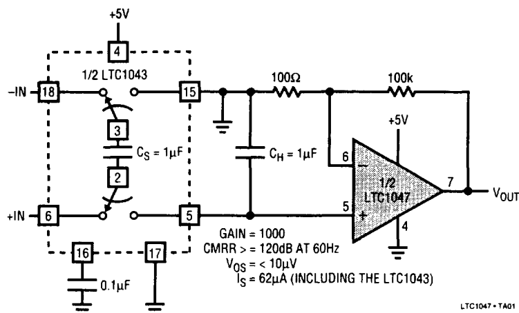
Micropower Single Supply Instrumentation Amplifier
