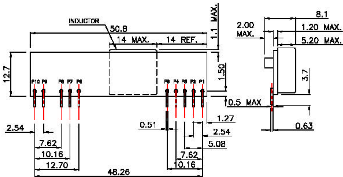
Figure 14. APA18 Mechanical Outline/ Drawing for Vertical type
