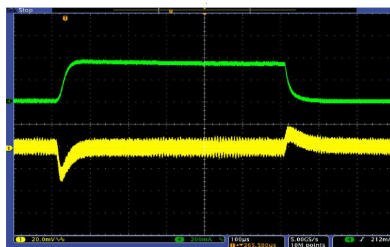
Figure 16. Load Transient Response, 10 mA to 350 mA
