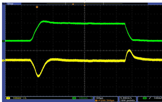
Figure 10. Load Transient Response, 10 mA to 200 mA
