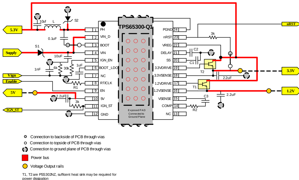
Figure 23. PCB Layout
