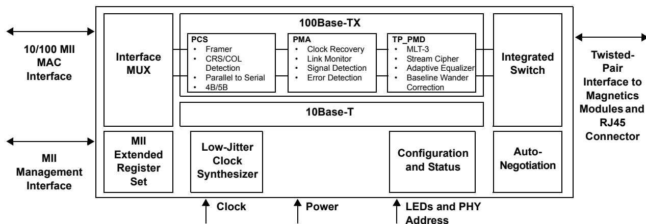
ICS1893AG Block Diagram
