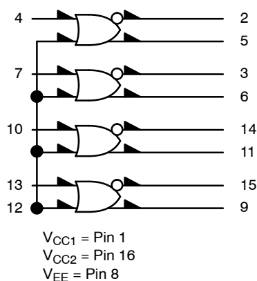
Figure 1. Logic Diagram
