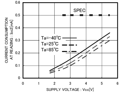
Fig.11 Current consumption at READ operation I_{CC2} ( f_{SCL}=400\text{kHz} )
