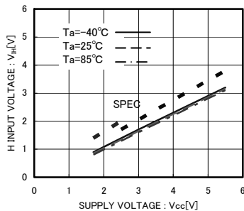
Fig.3 'H' input voltage V_{IH} (A0,A1,A2,SCL,SDA,WP)
