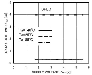
Fig.14 Data clock High Period t_{HIGH}
