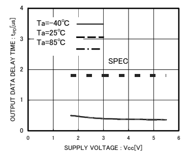
Fig.23 'H' Data output delay time t_{PD1}
