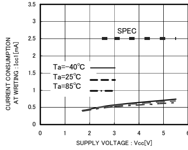
Fig.10 Current consumption at WRITE operation I_{CC1} ( f_{SCL}=400\text{kHz} BR24S128/256-W)
