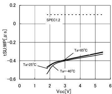
Fig.33 WP setup time t_{SU:WP}
