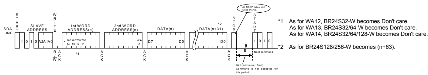
Fig.39 Page write cycle(BR24S32/64/128/256-W)
