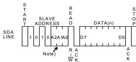
Fig.42 Current read cycle
