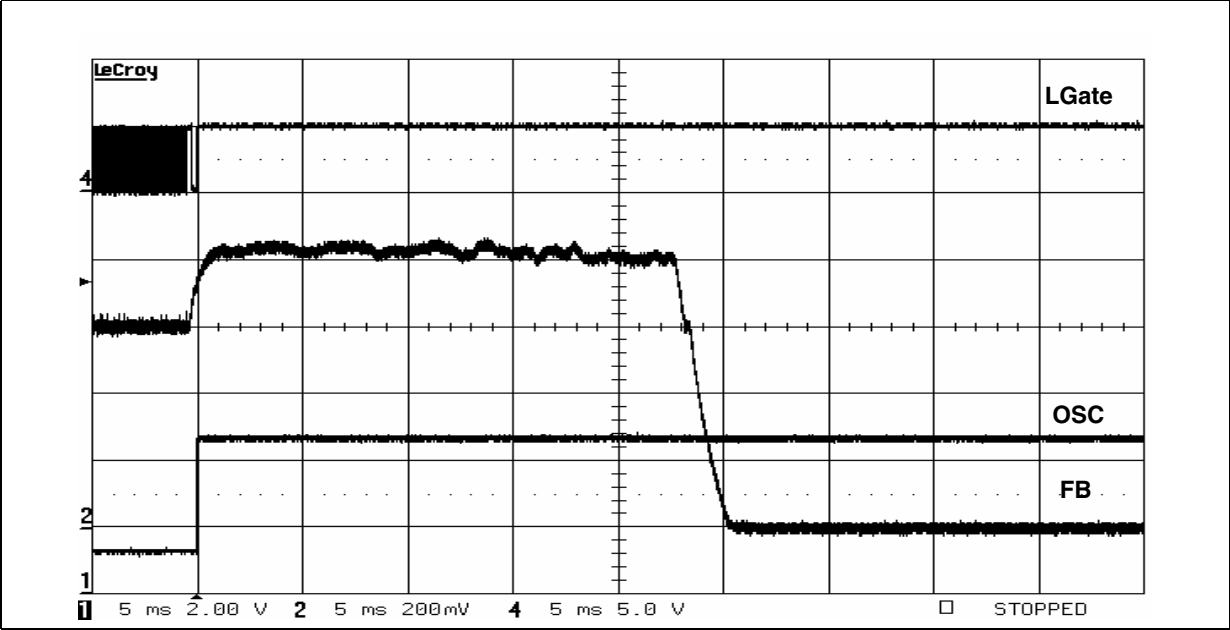
Figure 15. OVP latched
