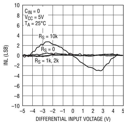
Figure 18. Measured INL vs Input Voltage, C_{IN} = 0 , V_{CC} = 5V , T_A = 25^\circ C
