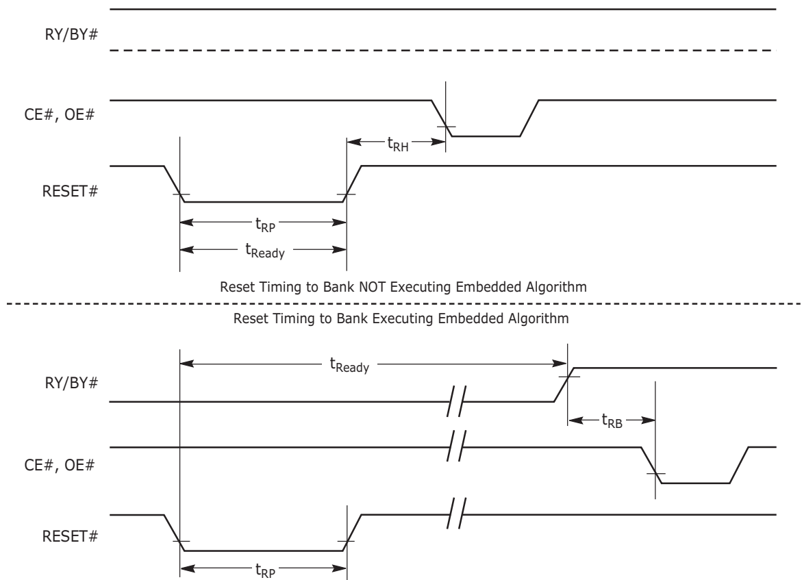
Figure 19. RESET# Timings
