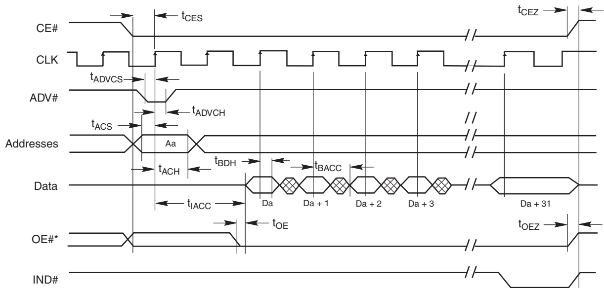
Figure I6. Burst Mode Read (x32 Mode)
