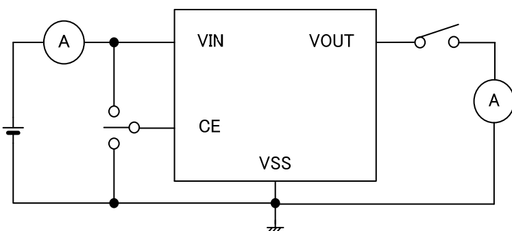
Circuit ③
