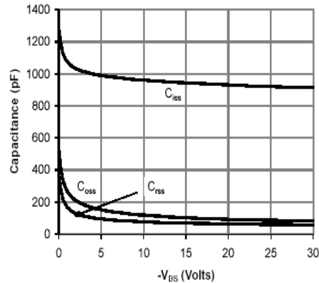
Figure 8: Capacitance Characteristics
