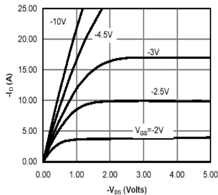
Fig 1: On-Region Characteristics
