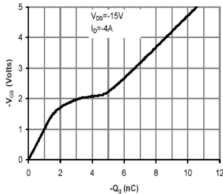
Figure 7: Gate-Charge Characteristics
