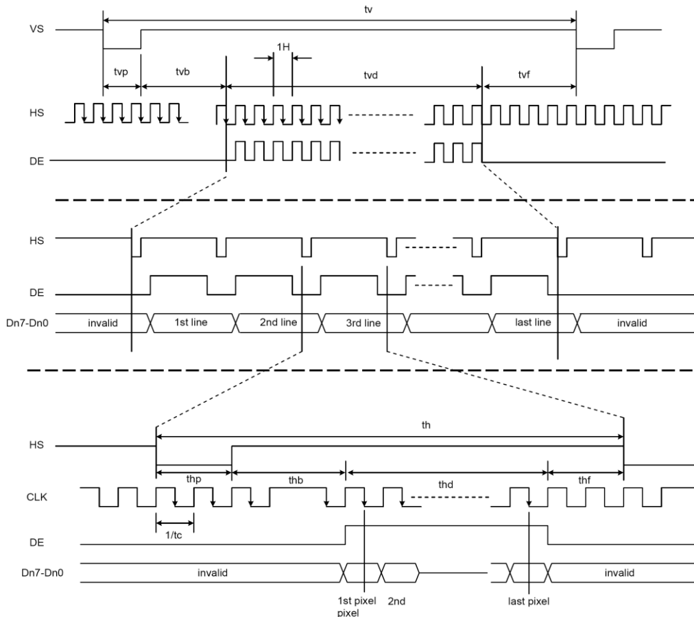
Figure 11.1 Input timing
