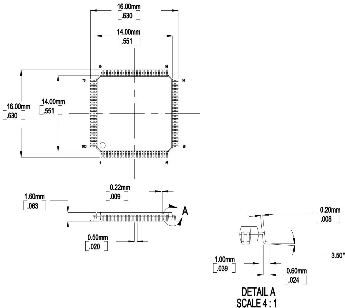
Figure 18: Mechanical Dimensions
