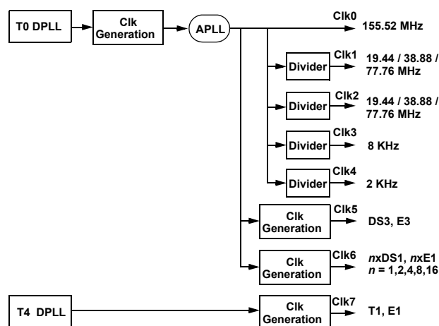
Figure 5: Output Clocks
