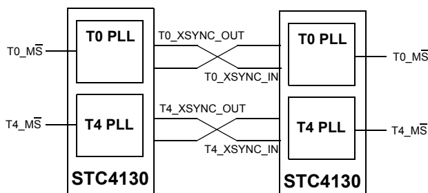
Figure 6: Master/Slave Configuration
