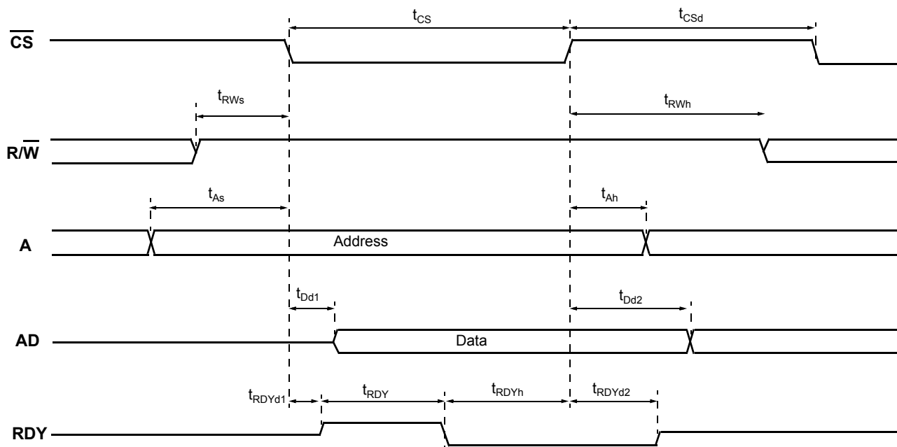
Figure 11: Motorola Bus Read Timing
