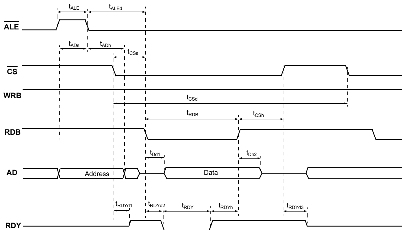
Figure 15: Multiplex Bus Read Timing
