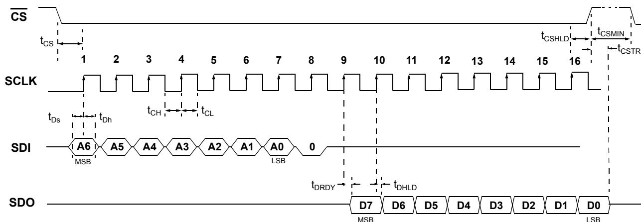
Figure 9: Serial Bus Timing, Read access
