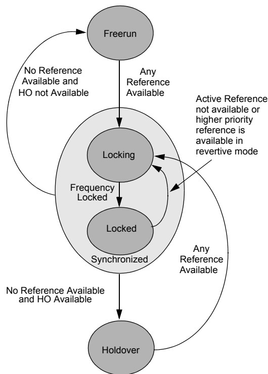
Figure 4: Device phase lock operational mode transi- tion in Automatic Reference Selection/Master Mode
