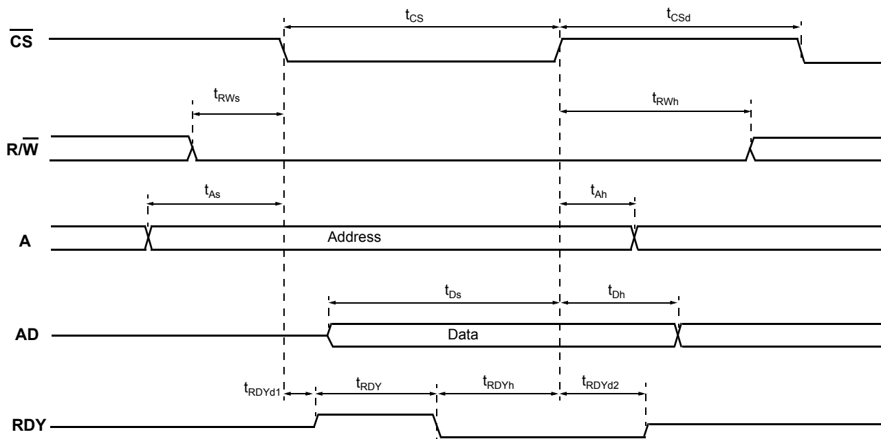
Figure 12: Motorola Bus Write timing
