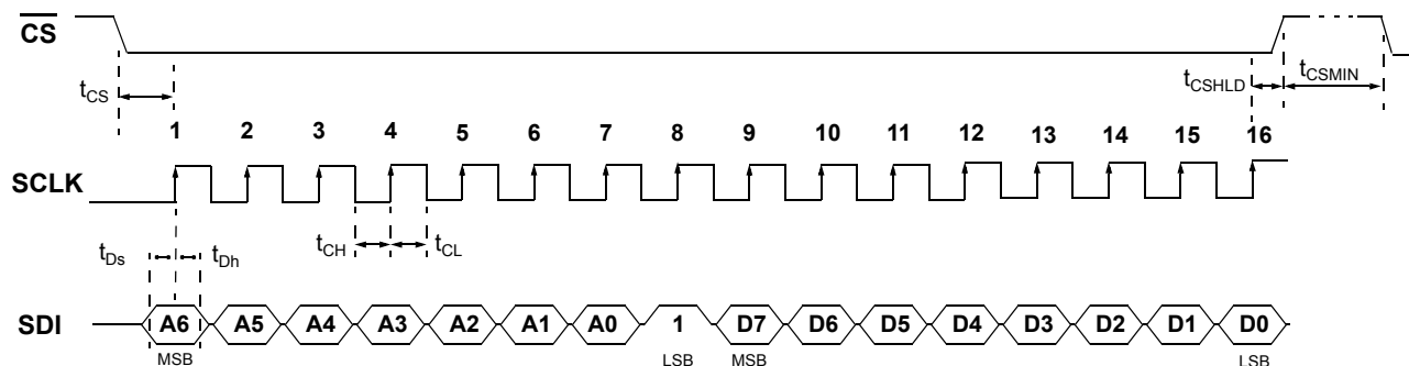
Figure 10: Serial Bus Timing, Write access
