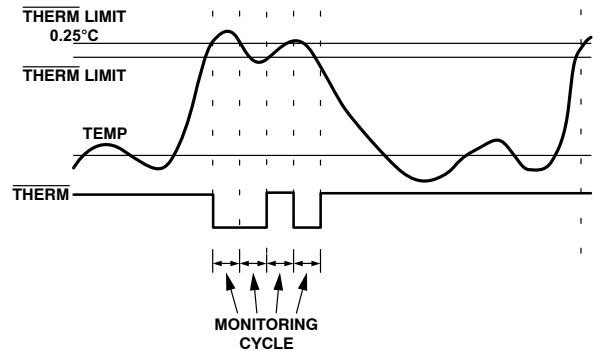
Figure 35. Asserting THERM as an Output, Based on Tripping THERM Limits
