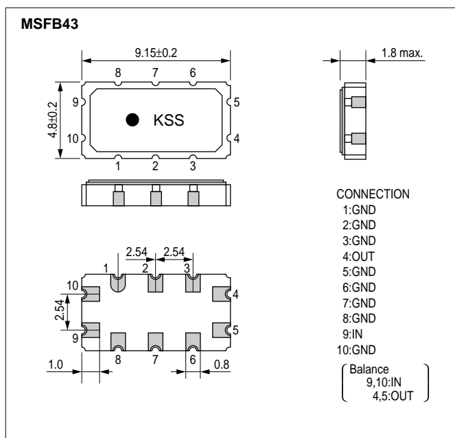
Dimensions(mm)
