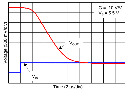
Figure 26. 正过载恢复
