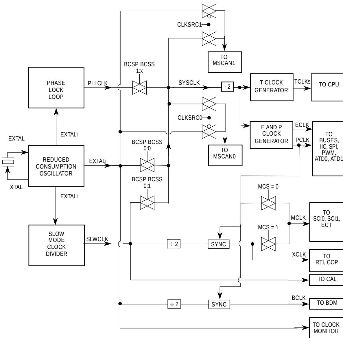
Figure 18 Clock Generation Chain
