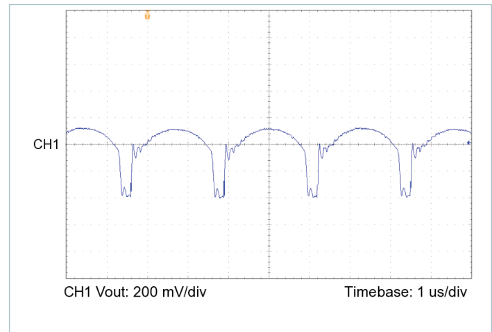
Figure 19 — Output voltage ripple, V_{IN} = 270\text{ V} , V_{OUT} = 3.3\text{ V} , C_{OUT\_EXT} = 1000\text{ μF} , R_{LOAD} = 0.073\text{ Ω}
