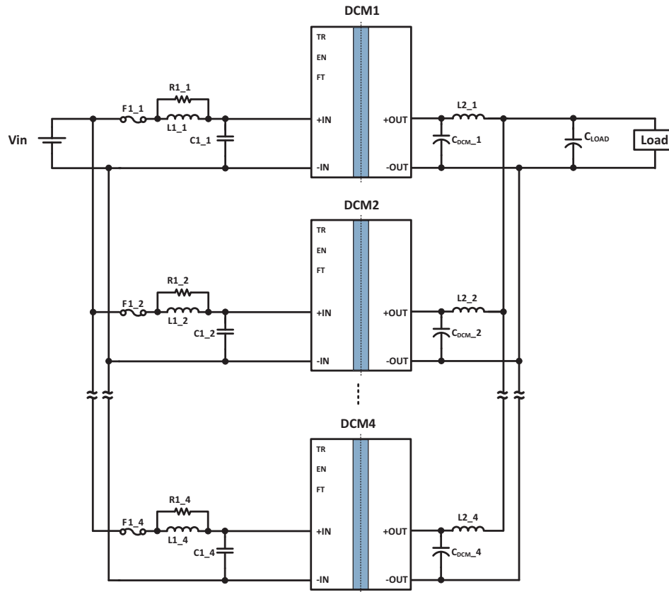
Typical Application 1: MDCM270P033M150A40 in an array of four units
