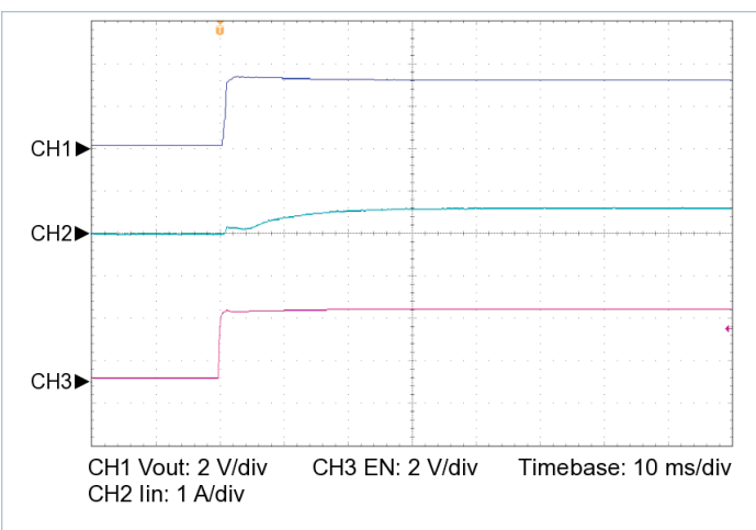
Figure 17 — Startup from EN, V_{IN} = 270\text{ V} , C_{OUT\_EXT} = 10000\text{ μF} , R_{LOAD} = 0.073\text{ Ω}
