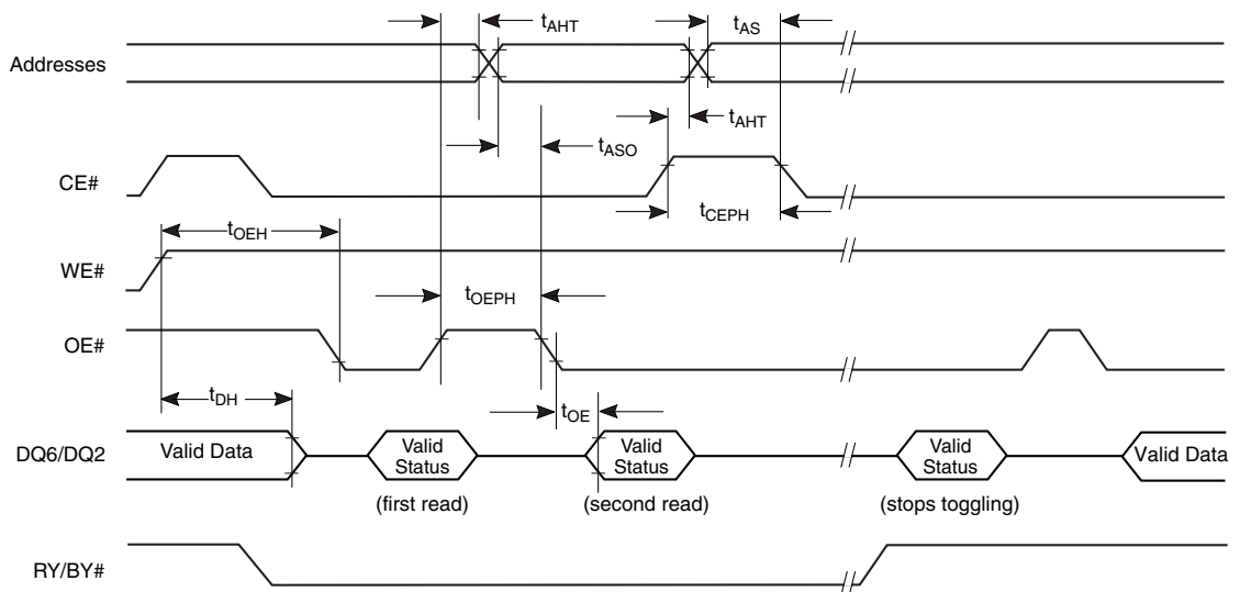
Figure II.I3 Data# Polling Timings (During Embedded Algorithms)
