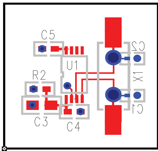
FIGURE 3B. 843001 PC BOARD LAYOUT EXAMPLE
