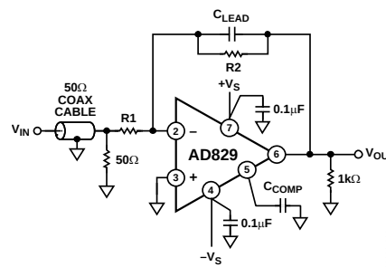
Figure 36. Inverting Amplifier Connection Using External Shunt Compensation
