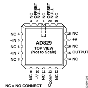
Figure 2. 20-Terminal LCC
