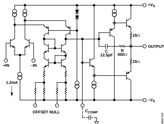
Figure 35. Simplified Schematic
