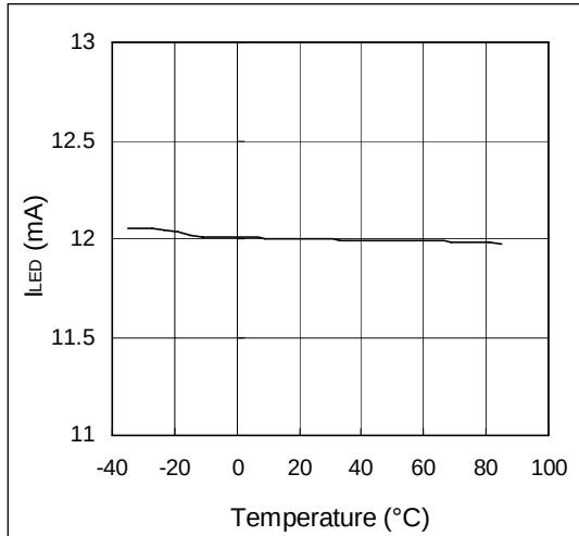
Figure 12. I_{LED} vs. Temp; V_{LED} = -0.25V , I_{SET} = 50\mu A
