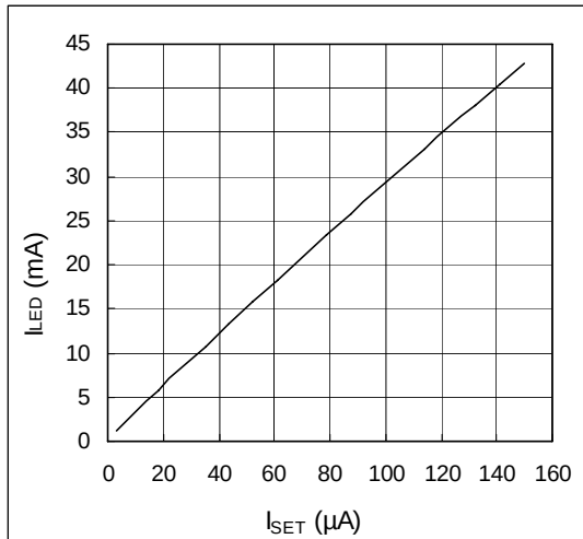
Figure 14. AS1102, AS1103, AS1104 I_{LED} vs. I_{SET}
