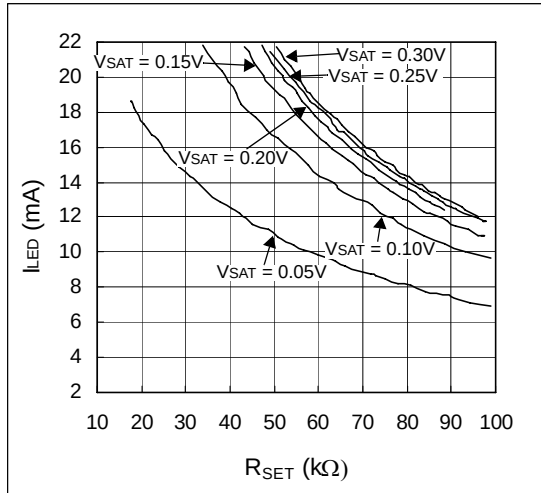
Figure 11. AS1101 I_{LED} vs. R_{SET} ; V_{SET} = 3V
