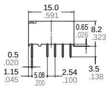
2 coil latching
