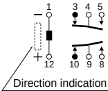
2 coil latching (Reset condition)
