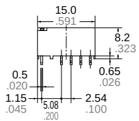
2 coil latching
