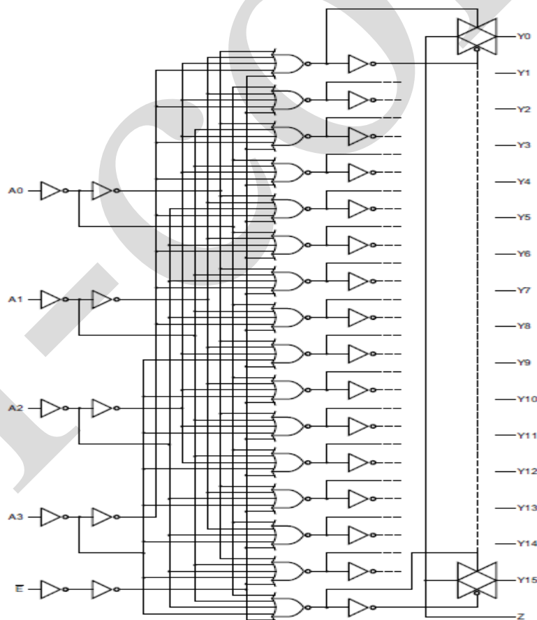
Figure 2. Logic diagram
