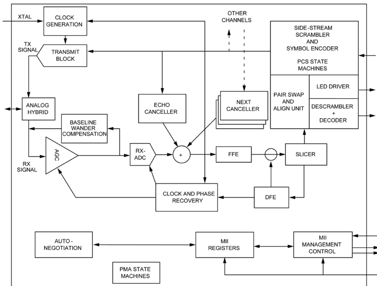
Figure 2. KSZ9031RX 1000Base-T Transceiver Block Diagram – Single Channel
