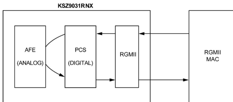
Figure 5. Local (Digital) Loopback
