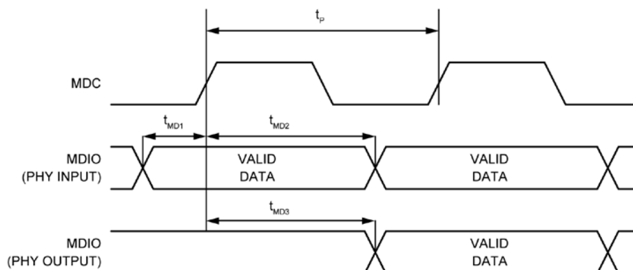
Figure 15. MDC/MDIO Timing
