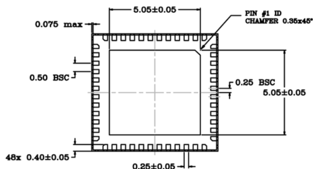
BOTTOM VIEW NOTE: 1, 2, 3, 7
