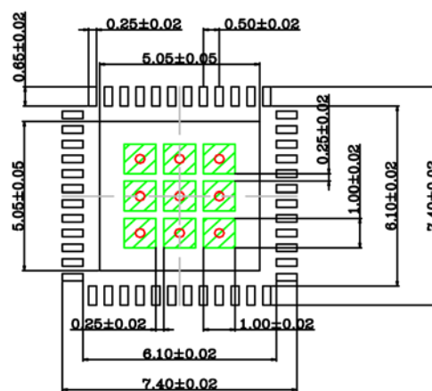
RECOMMENDED LAND PATTERN NOTE: 4, 5, 7
