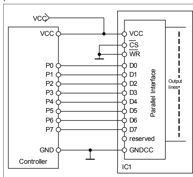
Figure 9 Parallel Direct Control
