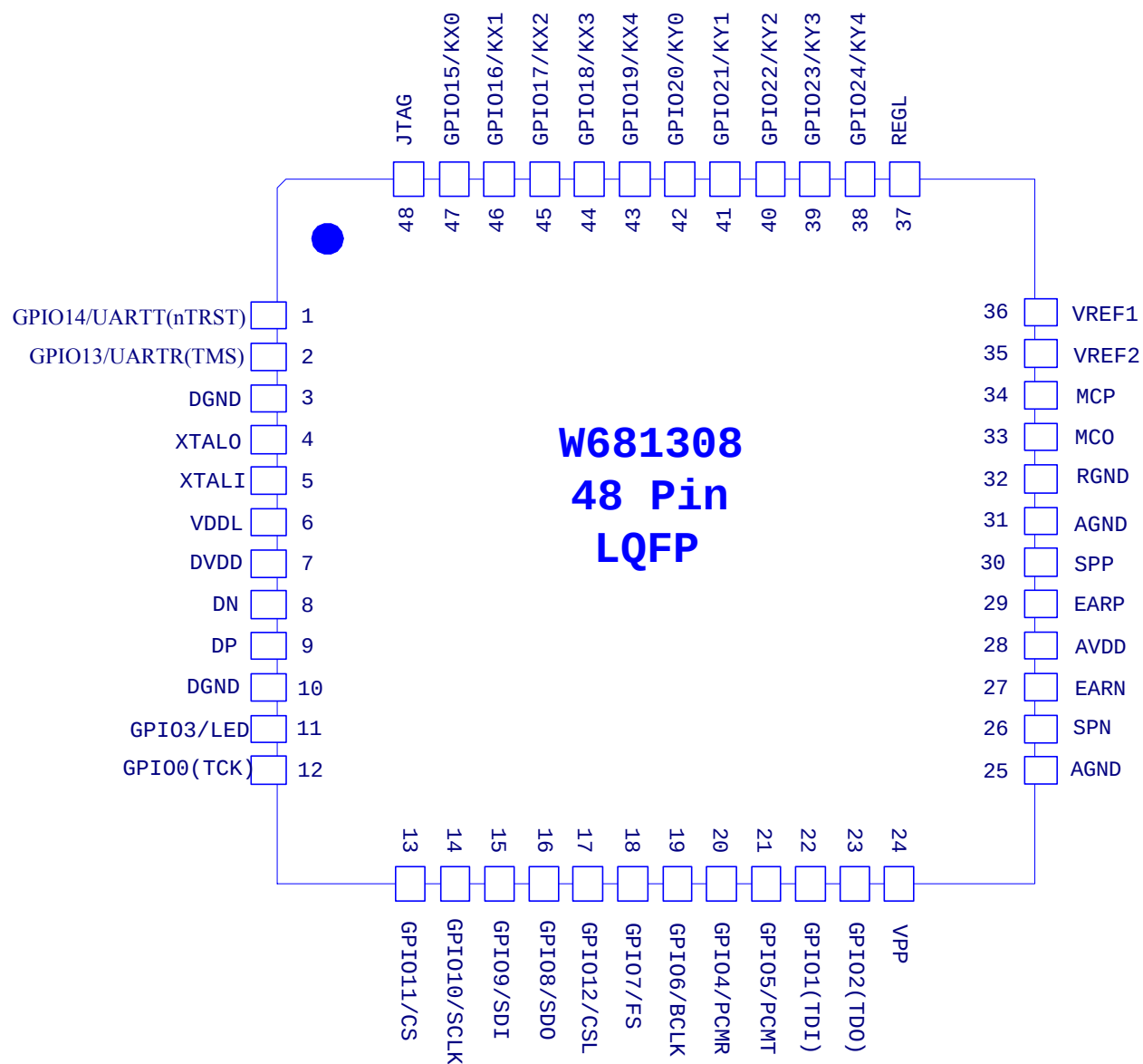
Figure 1 Pin diagram
