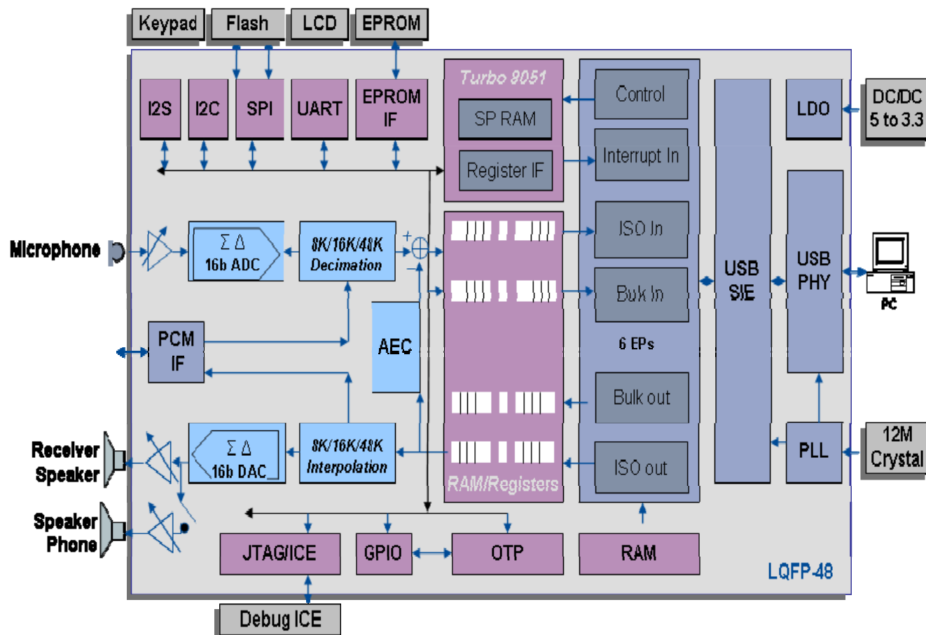
Figure 2 W681308 Function Block Diagram
