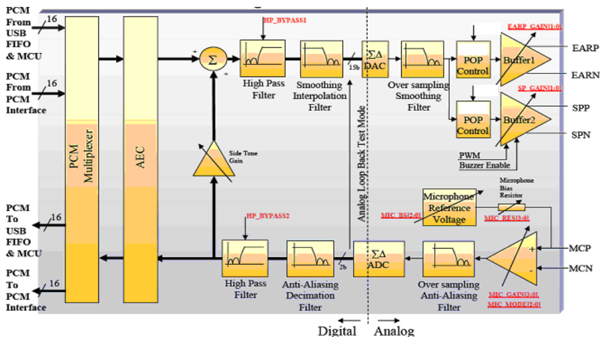
Figure 8 W681308 CODEC Signal Path Control
