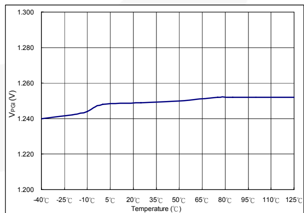
Figure 11. V_{PG1} vs. T_A
