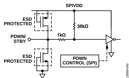
Figure 41. PDWN/STBY Input
