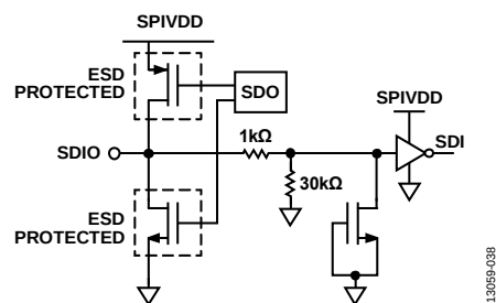
Figure 39. SDIO
