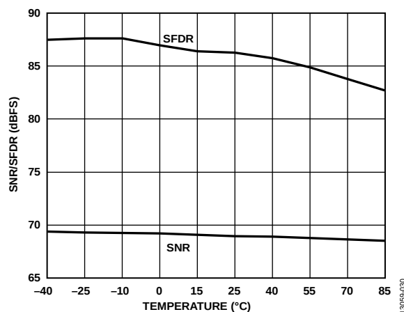
Figure 31. SNR/SFDR vs. Temperature, f_{IN} = 170.3 MHz
