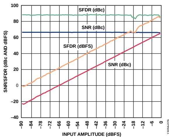
Figure 30. SNR/SFDR vs. Input Amplitude, f_{IN} = 170.3 MHz
