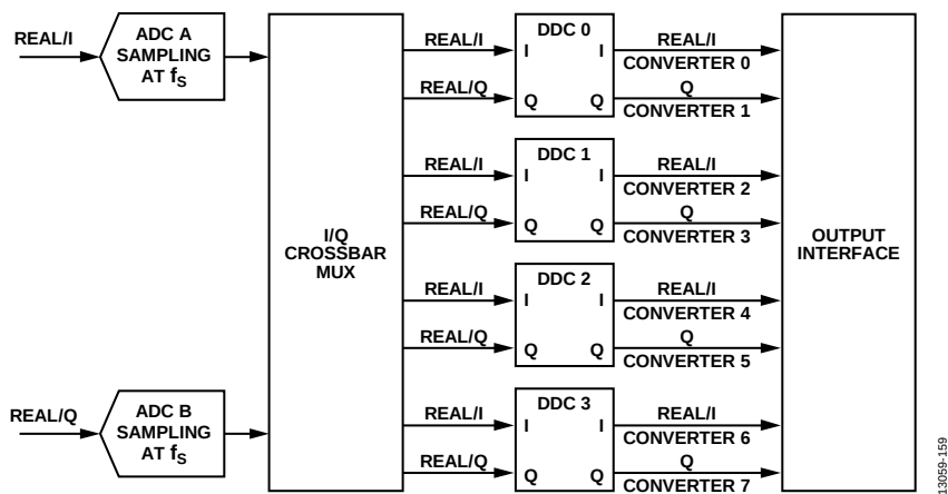
Figure 60. DDCs and Virtual Converter Mapping
