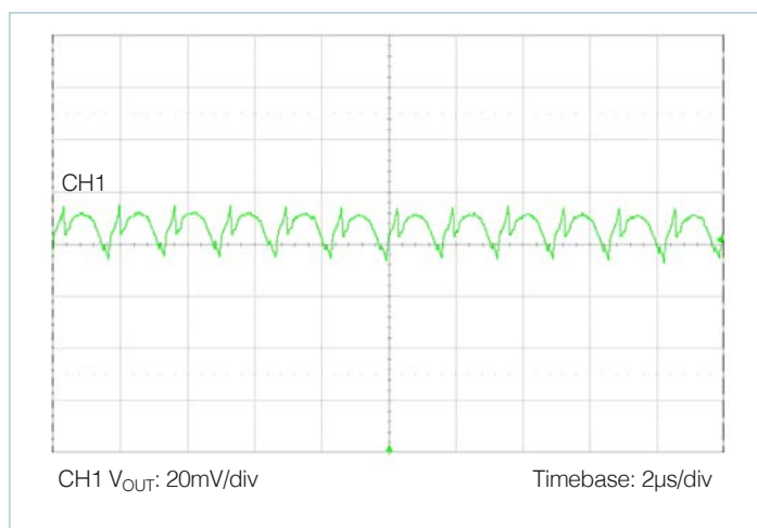
Figure 51 — Output voltage ripple: nominal line, nominal trim, 50% load, C OUT = 12 x 47µF ceramic
