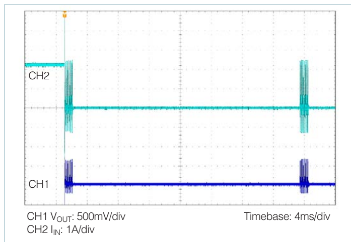
Figure 50 — Output short circuit, nominal line
