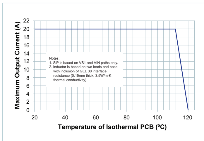
Figure 52 — System thermal specified operating area: max I OUT at nominal trim vs. temperature at locations noted
