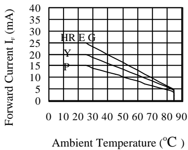
FIG.3 ALLOWABLE DC CURRENT VS. AMBIENT TEMPERATURE
