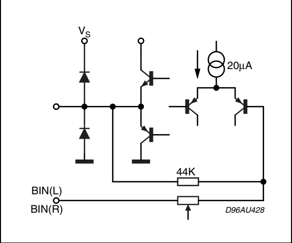
Figure 19. PINS: 12, 14
