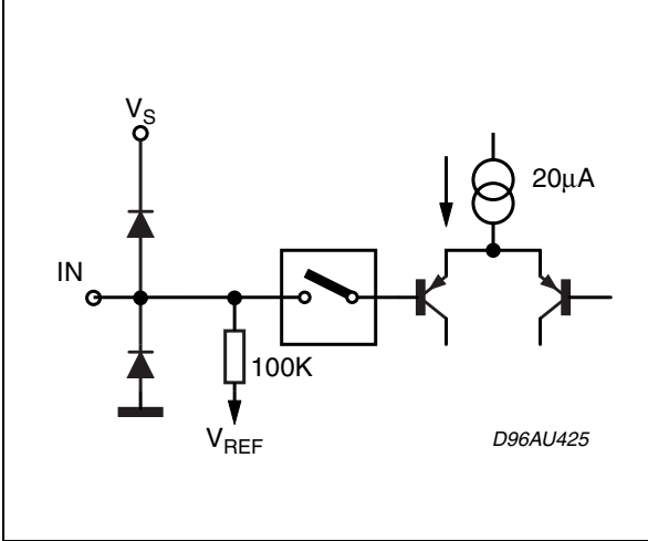
Figure 16. PINS: 1, 2, 3, 4, 5, 6, 7, 28
