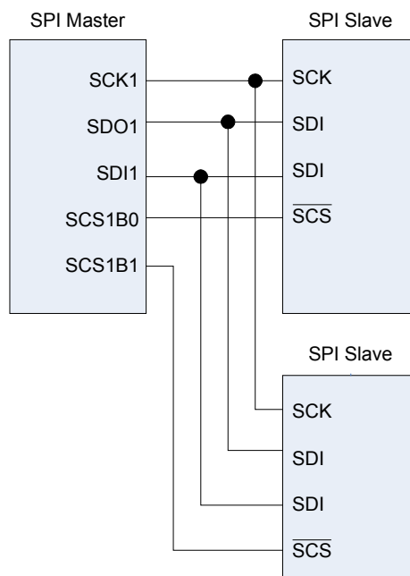
SPI1 Master/Slave Bus Connection
