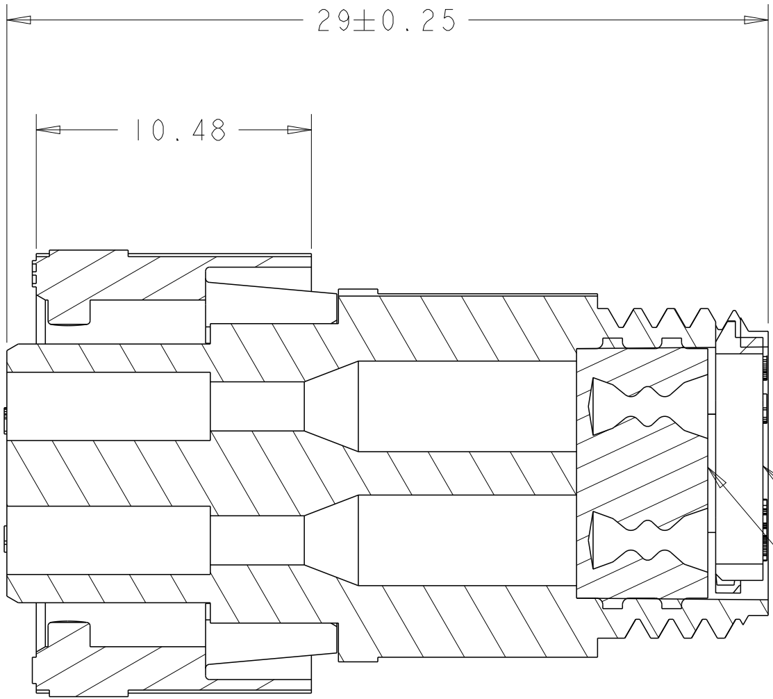
SECTION Z-Z
