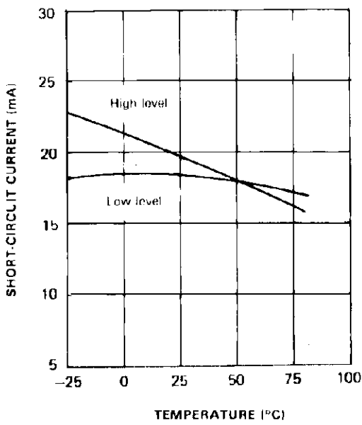
Figure 4: Short Circuit Current
