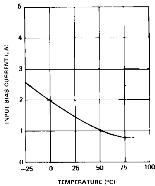
Figure 1: Input Bias Current
