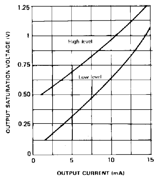
Figure 2: Output Saturation Voltage
