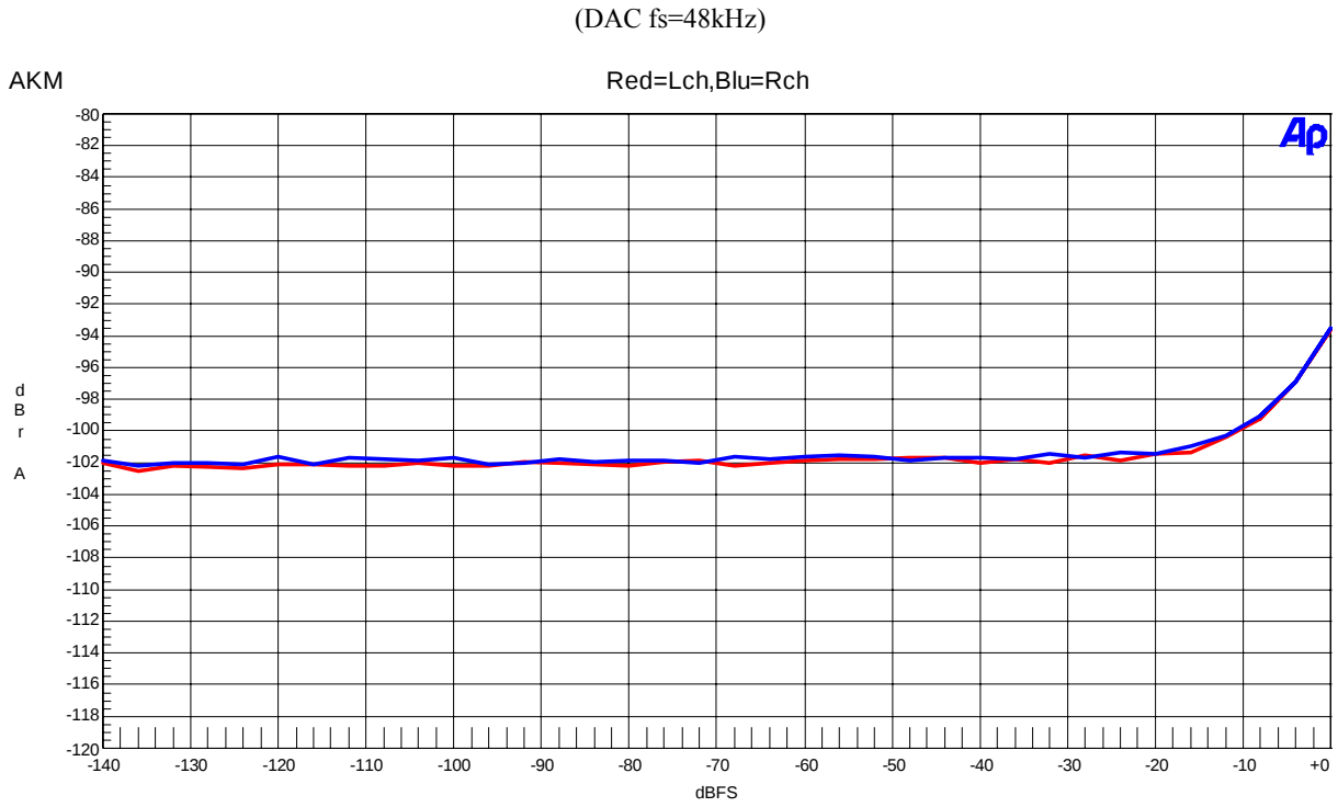
Figure 21. THD+N vs Input Level (Input Frequency=1kHz)
