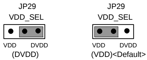
Figure 8. JP29 (VDD_SEL)
