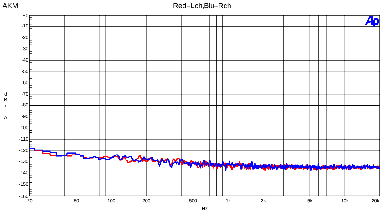
Figure 19. FFT(noise floor)
