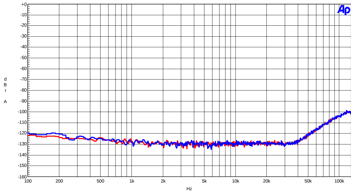
Figure 30. FFT (out-of-band noise)
