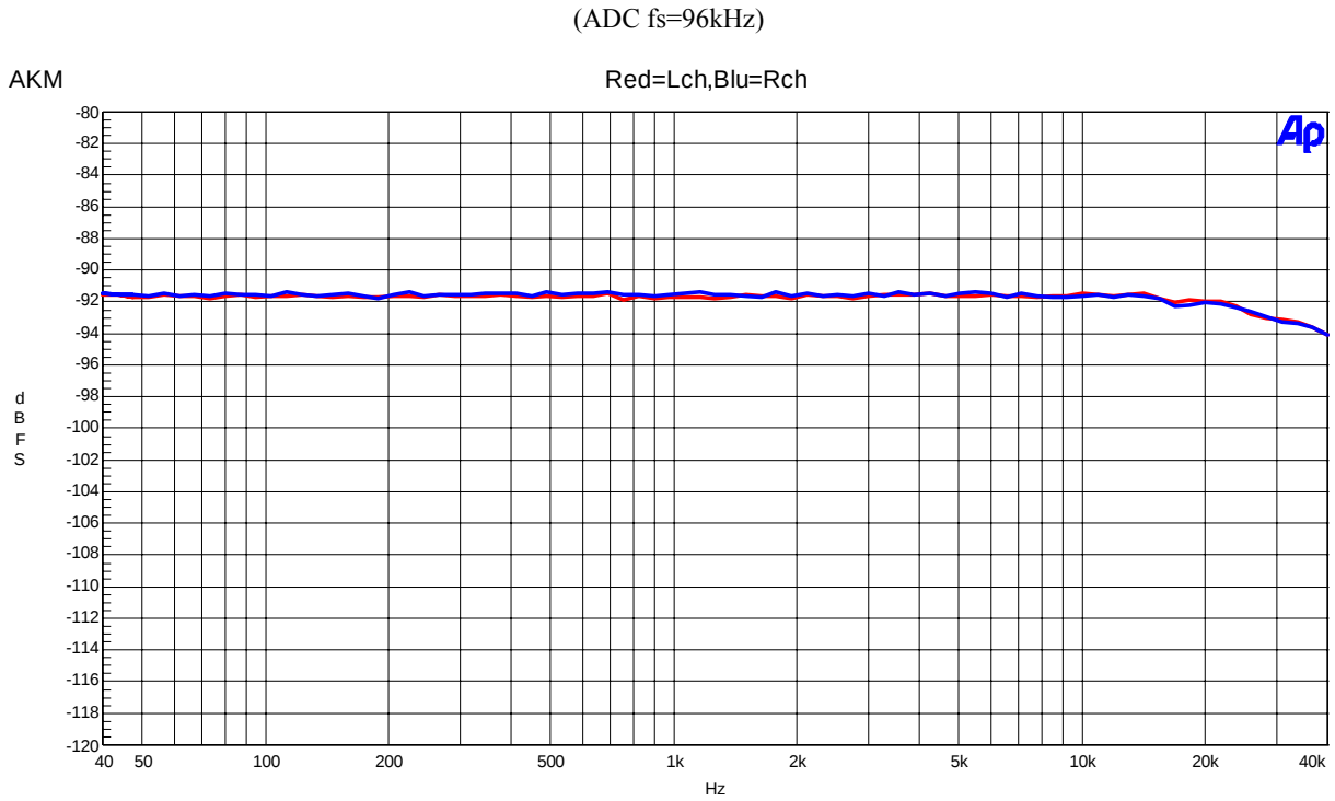
Figure 13. THD + N vs Input Frequency (Input Level=-0.5dBFS)
