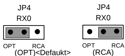
Figure 22. JP4 (RX0)
