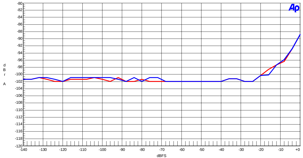
Figure 41. THD+N vs Input Level (Input Frequency=1kHz)
