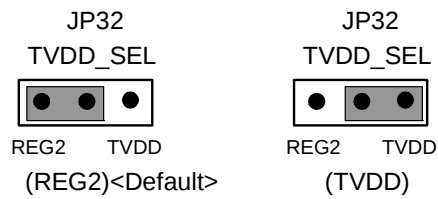
Figure 10. JP32 (TVDD_SEL)
