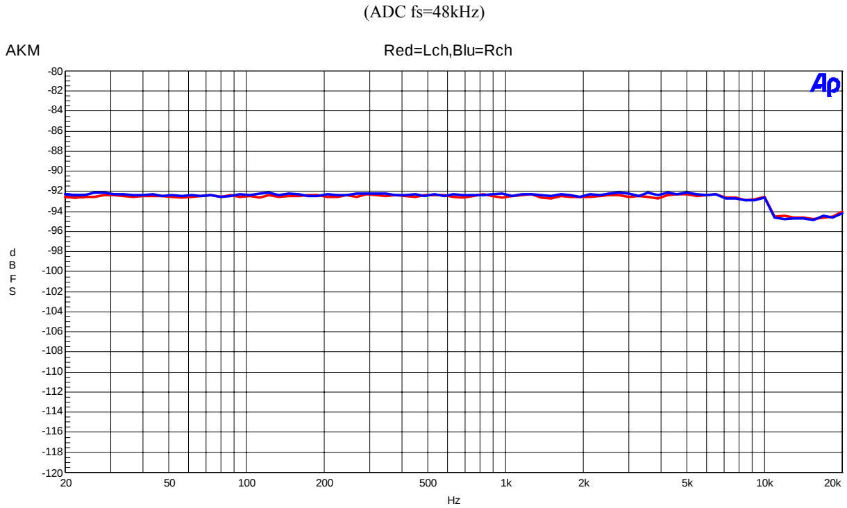
Figure 5. THD + N vs Input Frequency (Input Level=-0.5dBFS)
