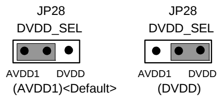
Figure 5. JP28 (DVDD_SEL)
