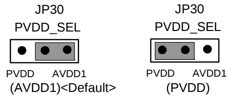
Figure 6. JP30 (PVDD_SEL)
