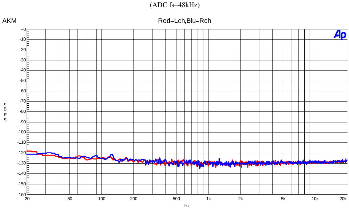
Figure 3. FFT(noise floor)
