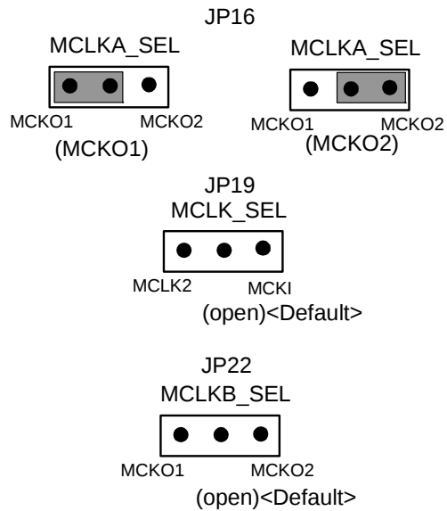
Figure 18. JP16 (MCLKA_SEL)
