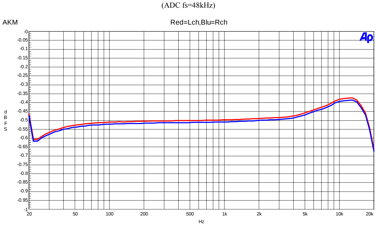
Figure 7. Frequency Response (Input Level=-0.5dBFS)
