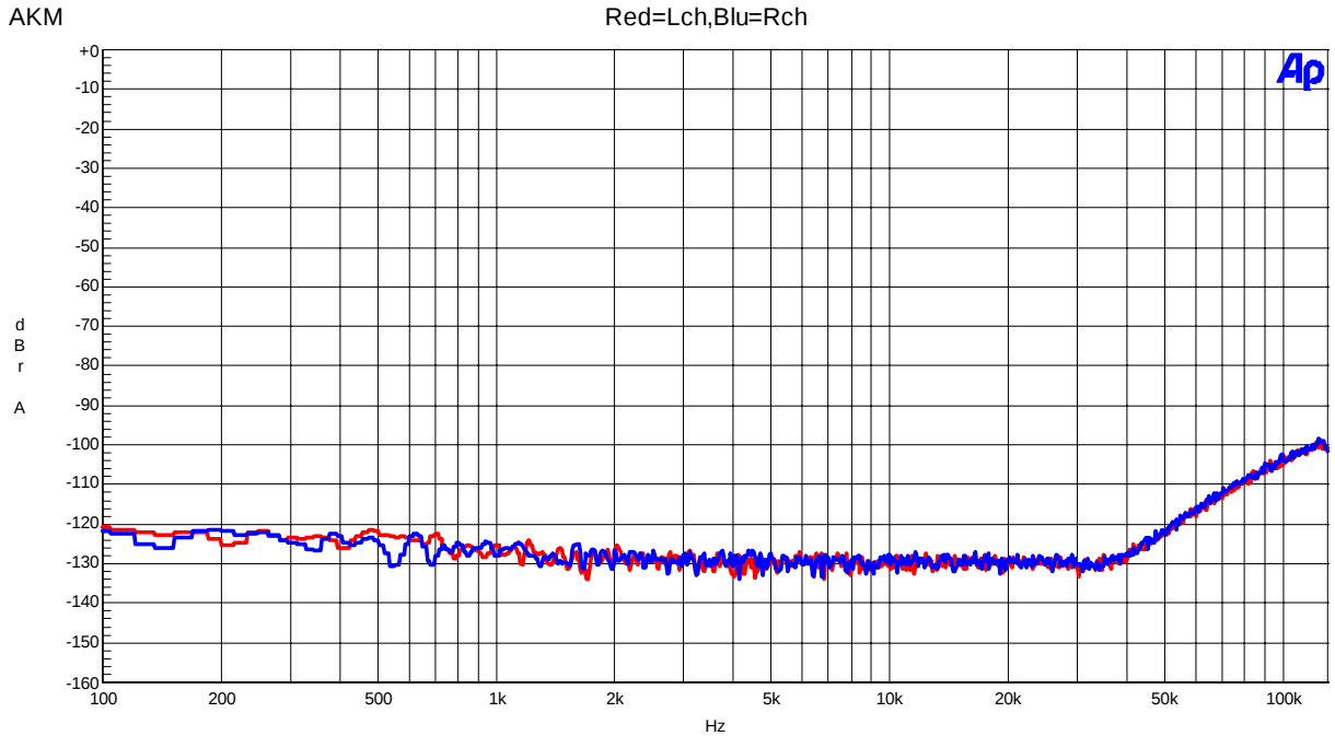
Figure 20. FFT(out-of-band noise)
