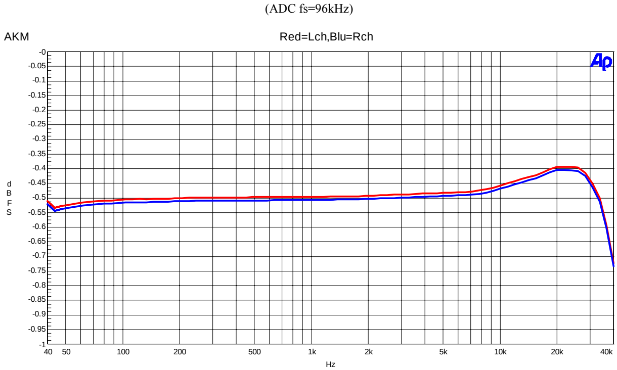
Figure 15. Frequency Response (Input Level=-0.5dBFS)
