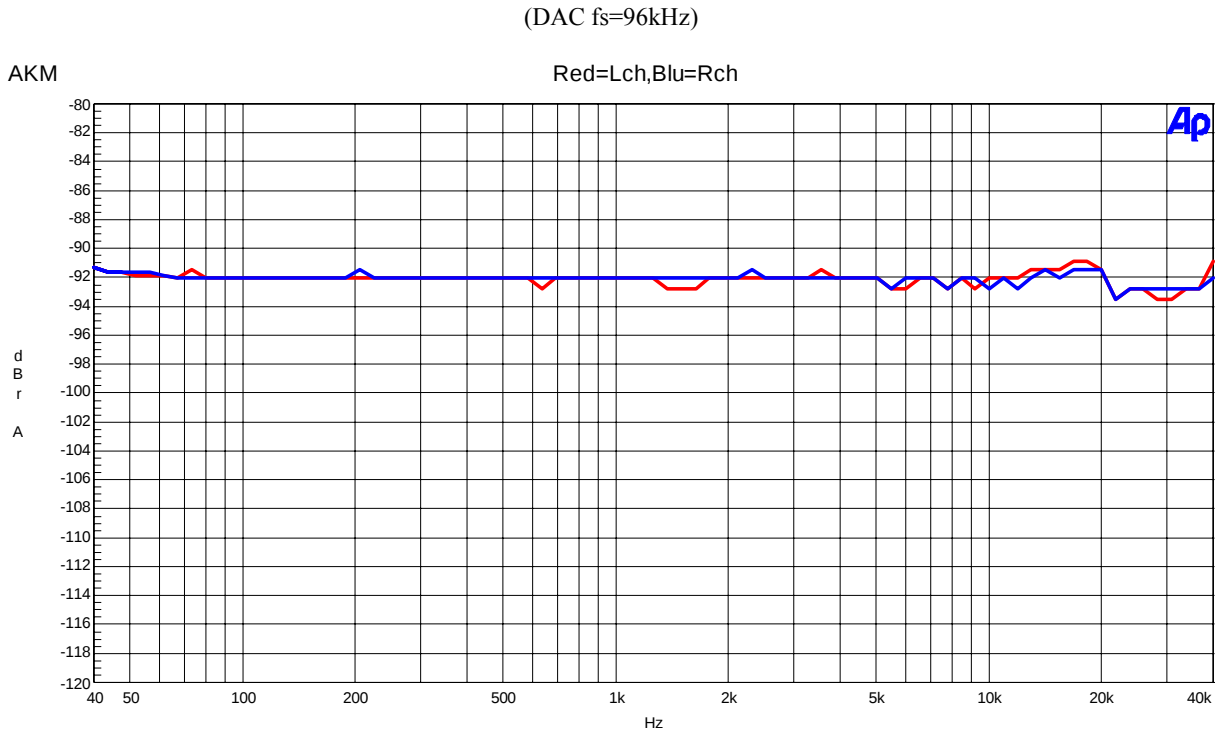
Figure 32. THD+N vs Input Frequency (Input Level=0dBFS)
