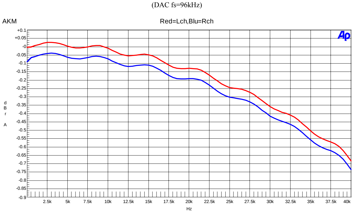
Figure 34. Frequency Response (Input Level=0dBFS)
