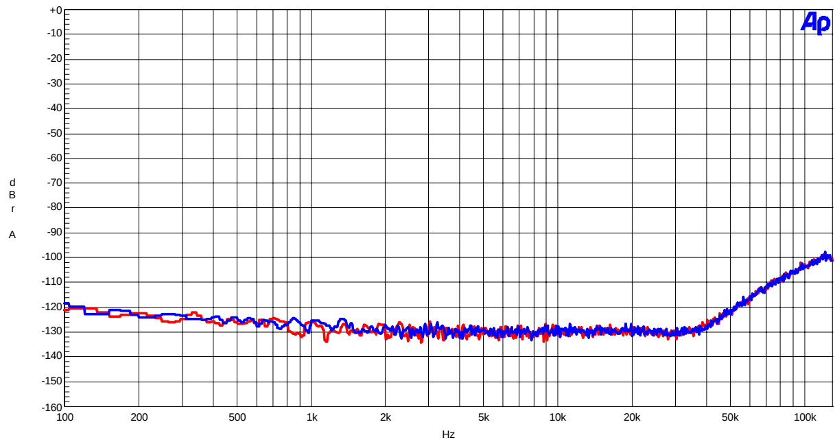
Figure 40. FFT(out-of-band noise)
