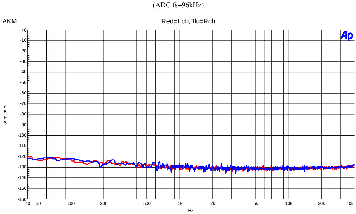
Figure 11. FFT(Noise floor)
