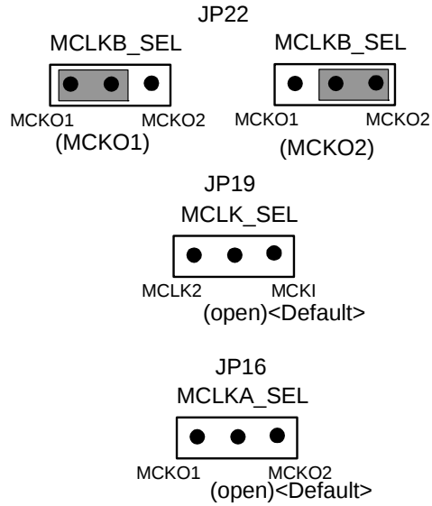
Figure 19. JP22 (MCLKB_SEL)
