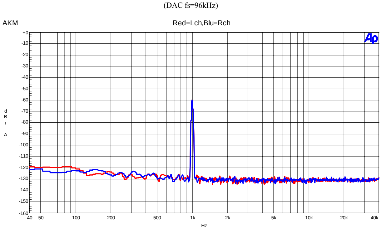
Figure 28. FFT(Input Frequency=1kHz, Input Level=-60dBFS)
