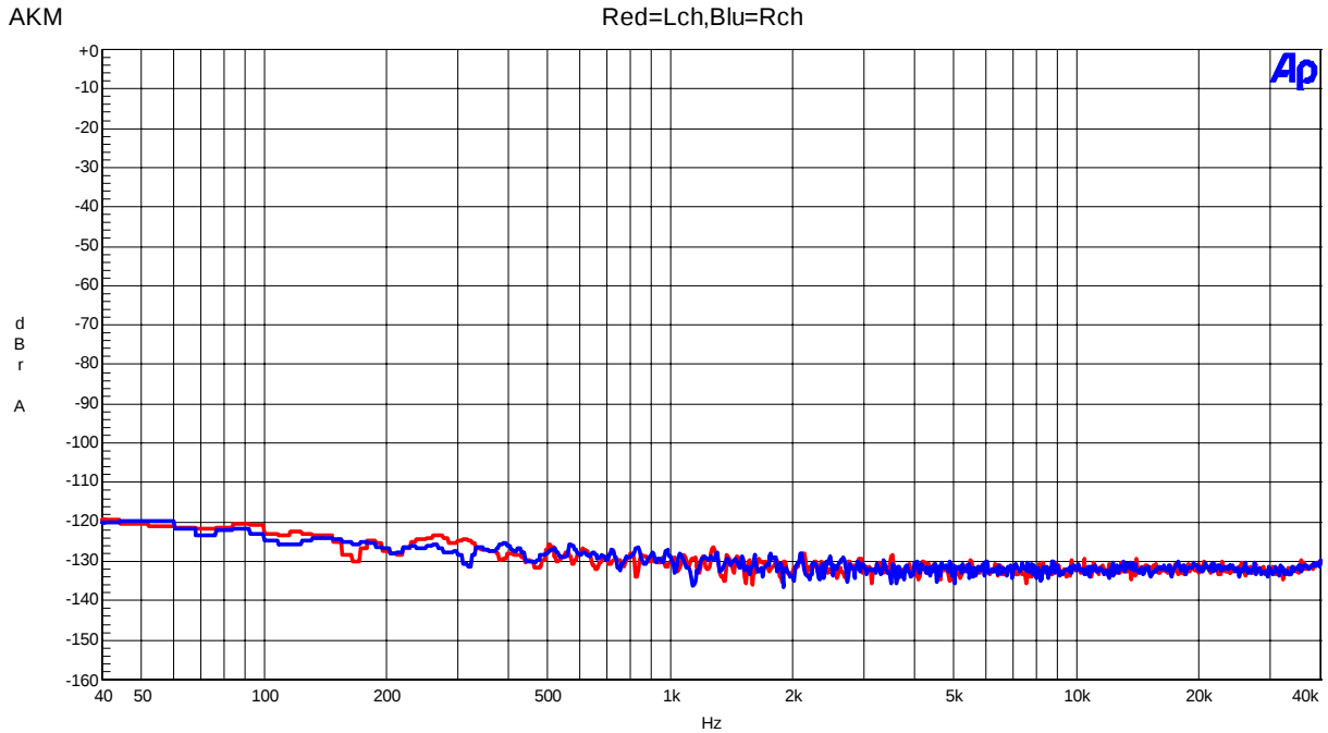
Figure 29. FFT(noise floor)
