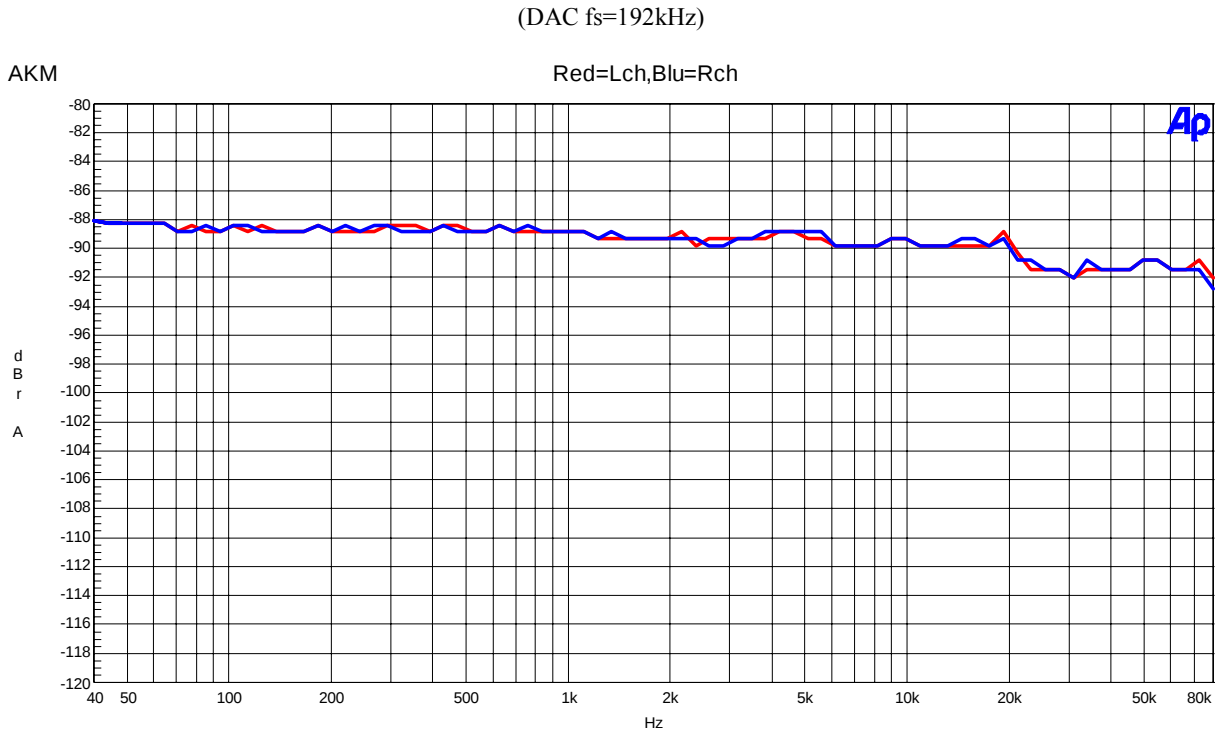
Figure 42. THD+N vs Input Frequency (Input Level=0dBFS)
