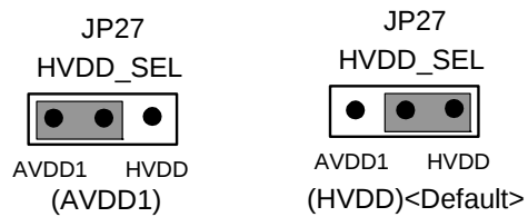
Figure 7. JP27 (HVDD_SEL)
