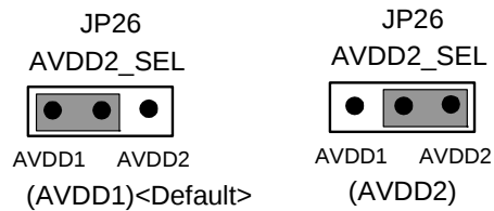
Figure 4. JP26 (AVDD2_SEL)
