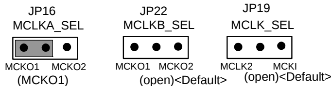
Figure 31. JP16 (MCLKA_SEL), JP22 (MCLKB_SEL), JP19 (MCLK_SEL)
