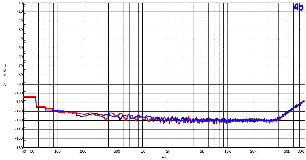
Figure 39. FFT(noise floor)
