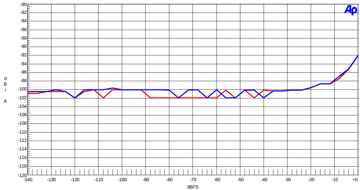
Figure 31. THD+N vs Input Level (Input Frequency=1kHz)
