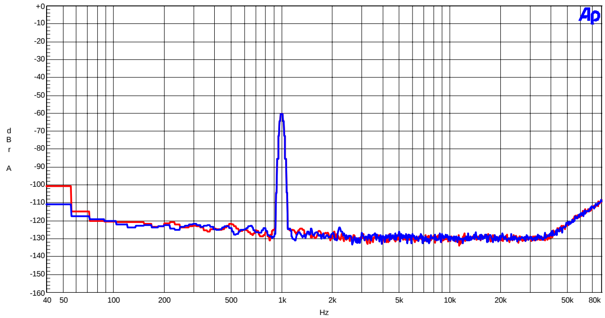
Figure 38. FFT(Input Frequency=1kHz, Input Level=-60dBFS)
