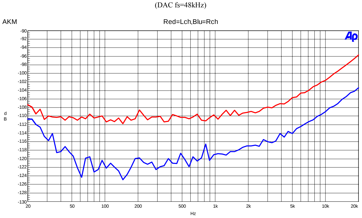
Figure 25. Cross-talk (Input Level=0dBFS)
