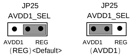
Figure 3. JP25 (AVDD1_SEL)
