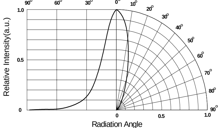
Radiation Characteristics
