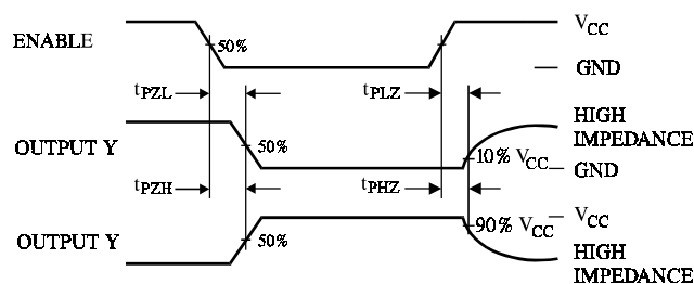
Figure 2. Switching Waveforms
