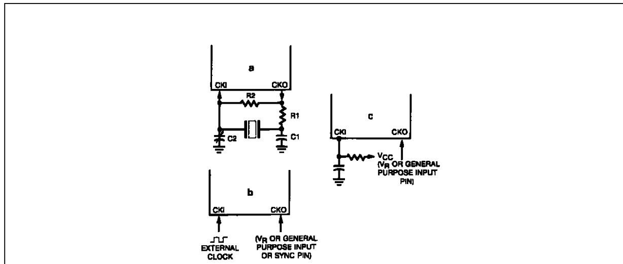
Figure 4 : ETL9444/L9445 Oscillator.
