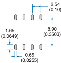
Recommended PCB Land Pattern
