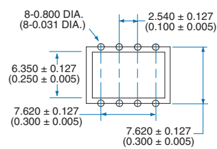
PC Board Pattern
