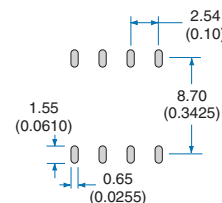
Recommended PCB Land Pattern
