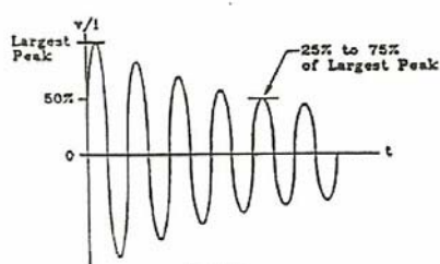
FIGURE 7 – Waveform 3
