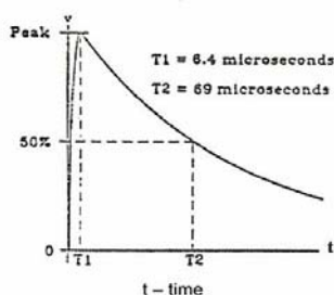
FIGURE 8 – Waveform 4
