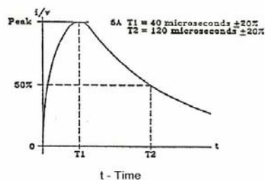
FIGURE 9 – Waveform 5A
