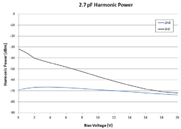
Figure 3. Harmonic Power
