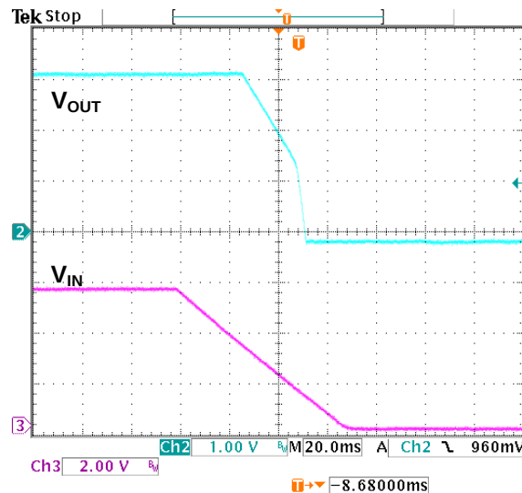
Figure 11. Power off Response
