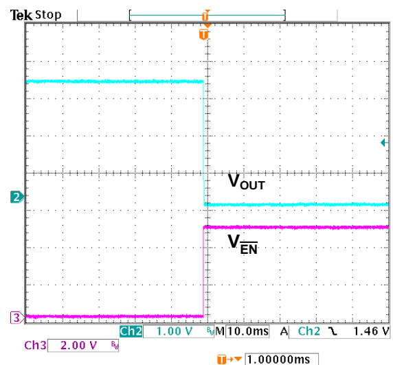
Figure 13. \overline{EN} Shutdown Response
