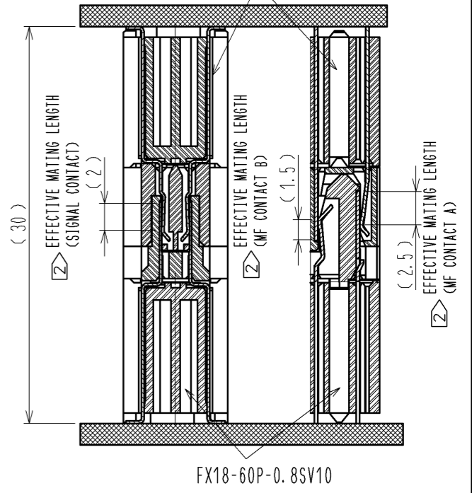
CROSS SECTION OF MATING(FREE) STACKING HEIGHT=30mm FX18-60S-0.8SV20
