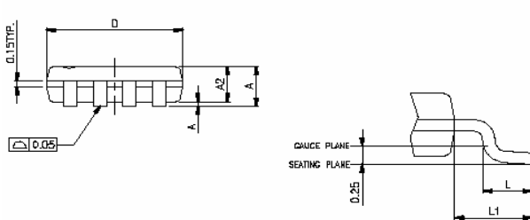
(F75386M 8-MSOP Package)
